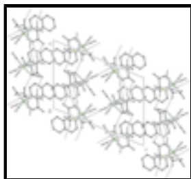
Fig. 3. A view down [010] of a section of (I) with intermolecular hydrogen bonding contacts of the columns indicated by dashed lines.
