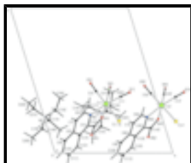
Fig. 2. A view of the independent molecules down [100] indicating the superstructure effect (translation t ) along the b -axis.
