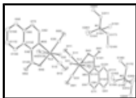
Fig. 1. A view of the molecular structure of (I) with displacement ellipsoids for the non-hydrogen atoms drawn at the 30% probability level (H atoms omitted for clarity).
